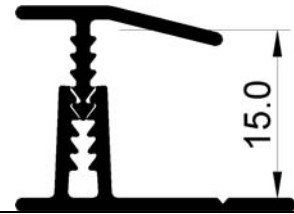
ETPE9/15T (top part) & ETPE9/15B (bottom part) – Two part adjustable edge strip. 9mm – 15mm boarding. (Scale 2:1)
