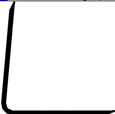
EA50EXT – 50mm External Angle. (Scale 1:1)
